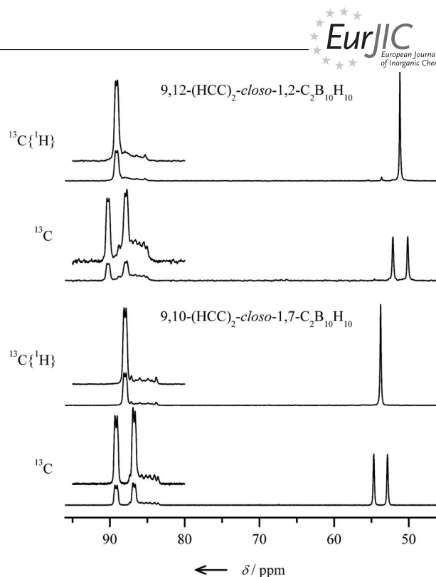
Figure 5. ^{13}\text{C} and ^{13}\text{C}\{^1\text{H}\} NMR spectra of 9,12-(HCC) 2 - closo -1,2- \text{C}_2\text{B}_{10}\text{H}_{10} ( 1a ) and 9,10-(HCC) 2 - closo -1,7- \text{C}_2\text{B}_{10}\text{H}_{10} ( 3a ).
